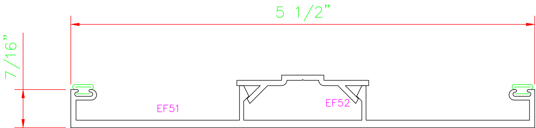
EF51 / EF52 5 1/2" X 7/16" MULLION COVER & CLIP
